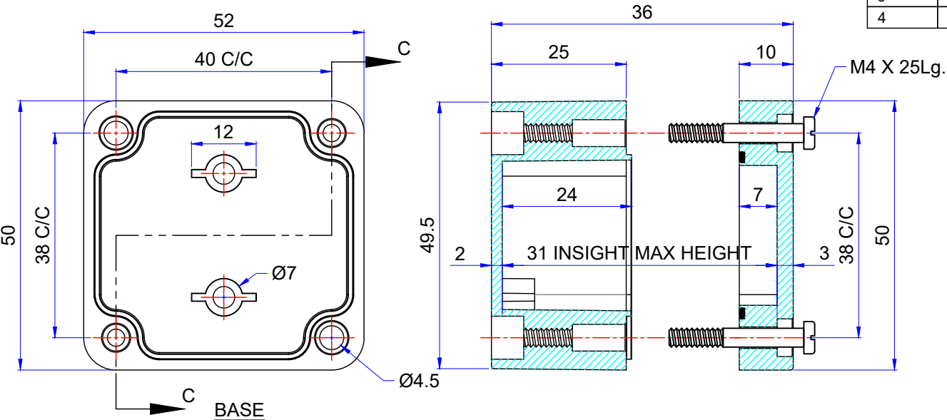
SECTION C-C
